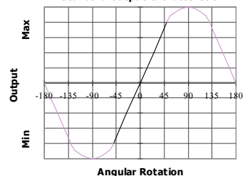
Direction of increasing output in calibrated sector Standard Output Characteristic
